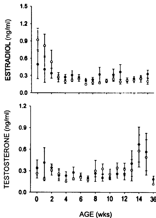
FIG. 2. Circulating levels of endogenous E_2 and T in intact neonatal red-spotted garter snakes from birth to 15 weeks and at the 36th week. Values are means \pm SE. Males are represented by closed circles ( n = 10 for each week). Females are represented by open circles ( n = 10 for each week).
