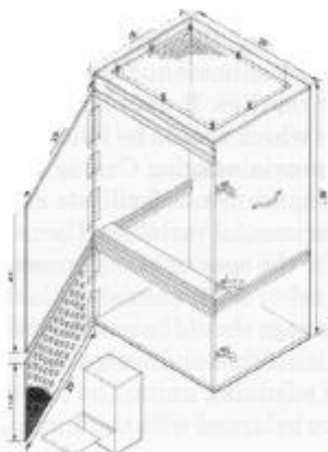
Figure 2 Schematic of cage design showing details of hardware. Inset demonstrates the insertion of the aluminum panel.
